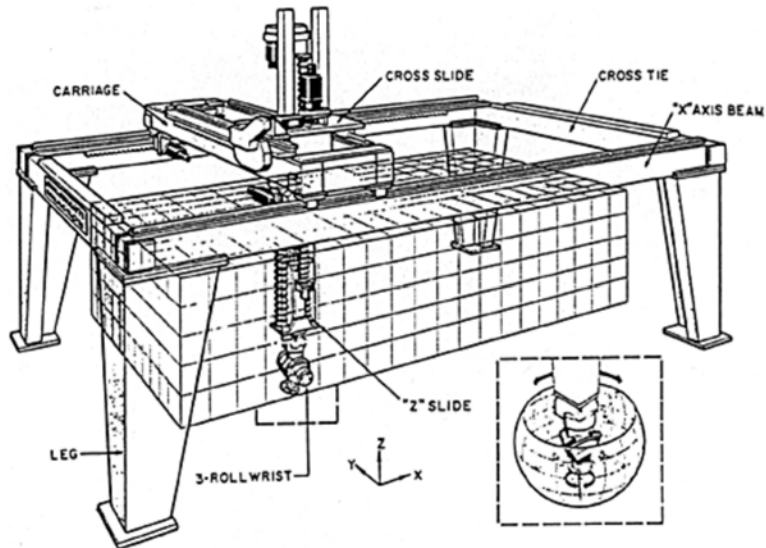
Figure B-1 Cartesian Robot
