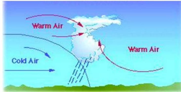
Figure 1 Cold Front
