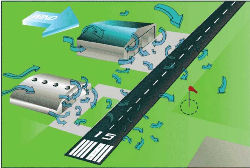
Figure 6 Mechanical Turbulence
