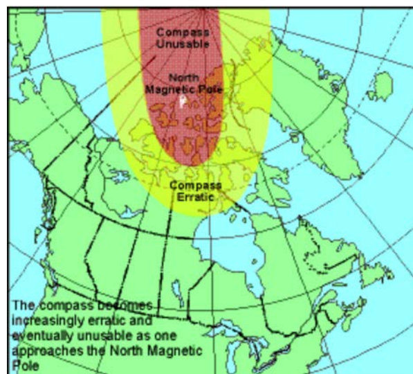
Figure 1 Earth's Magnetic Field
