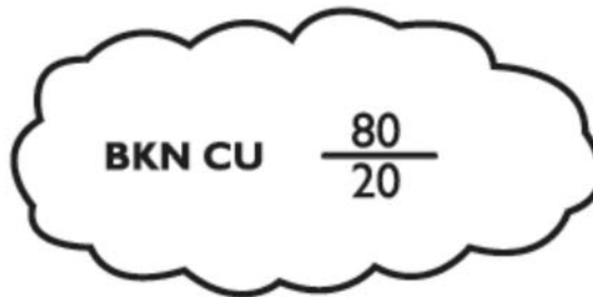
Figure J-1 Synoptic Features
