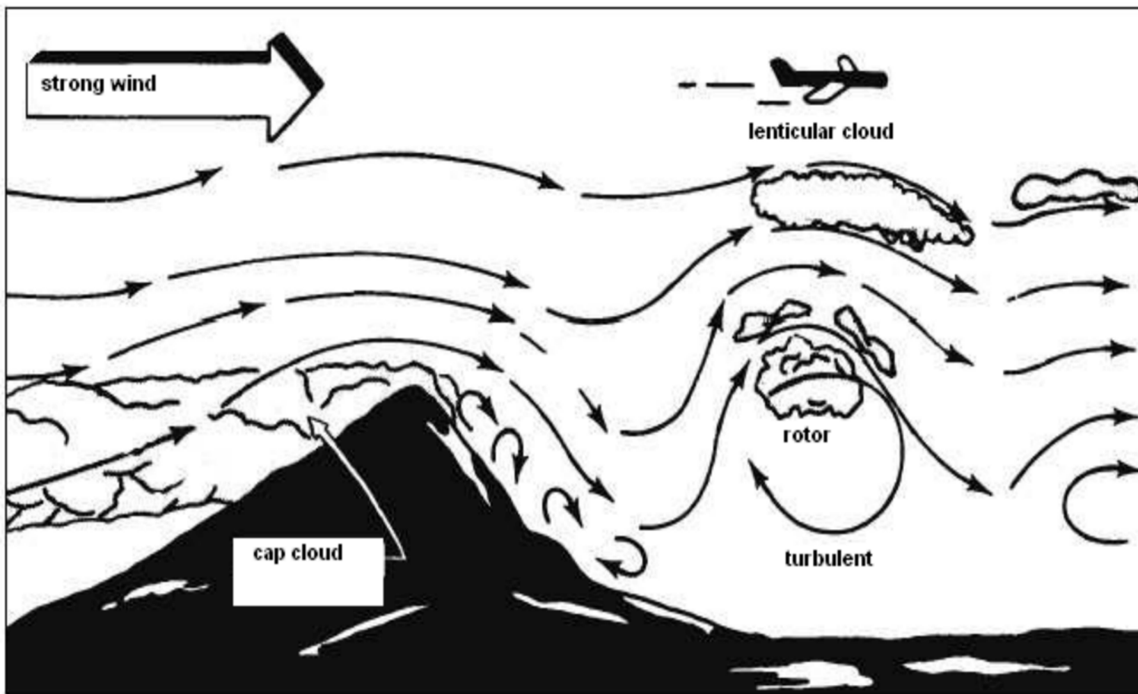
Figure A-3 Mountain Wave
