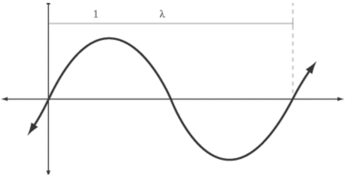
Figure A-1 Transverse Wavelength
