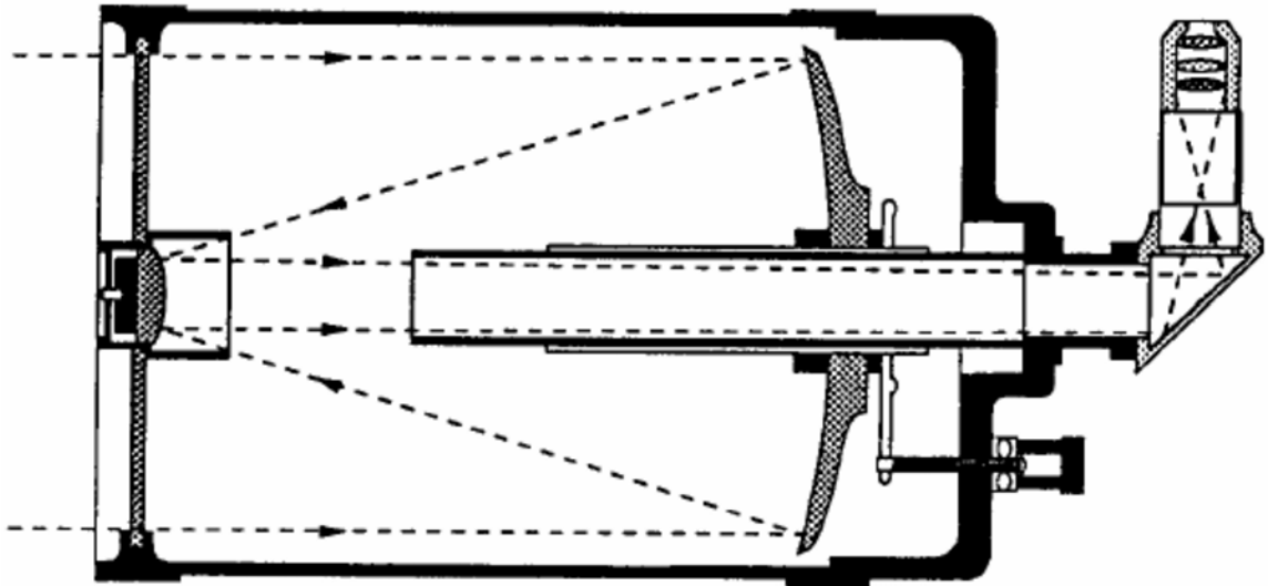
Figure B-1 Schmidt-Cassegrain Telescope Design
