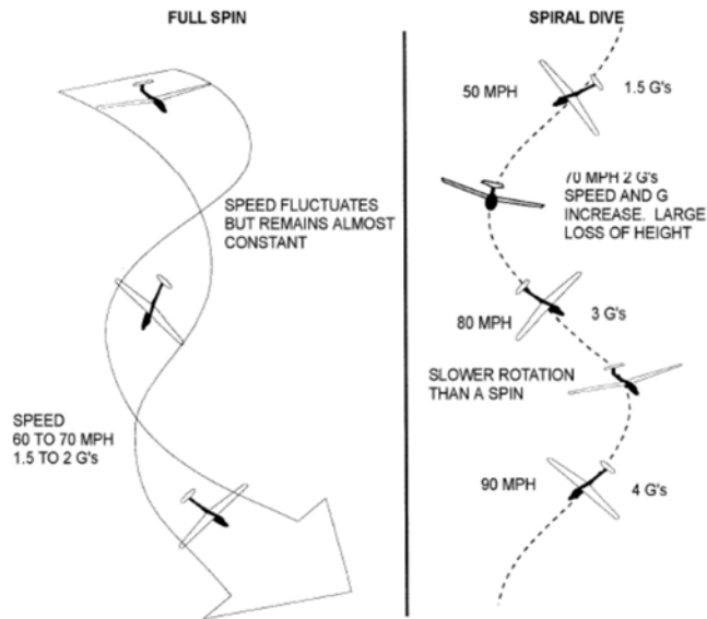
Figure A-11 Spin
