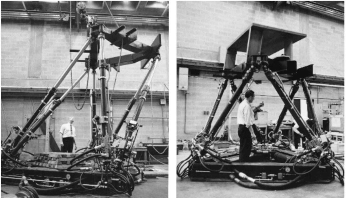
Figure B-7 Parallel Robot
