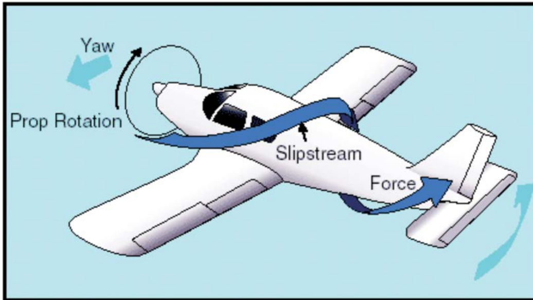
Figure A-3 Precession When the Tail is Lifted
