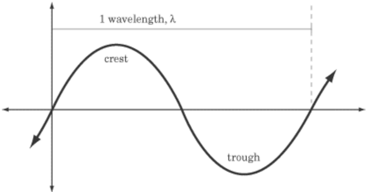
Figure B-1 Transverse Wavelength
