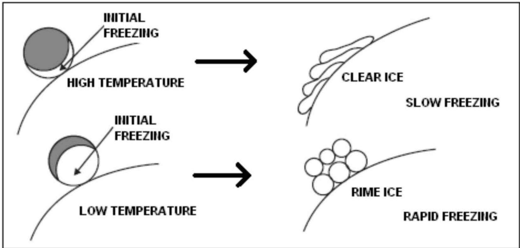
Figure A-3 Clear Ice and Rime Ice
