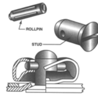
AIRLOC FASTENER
