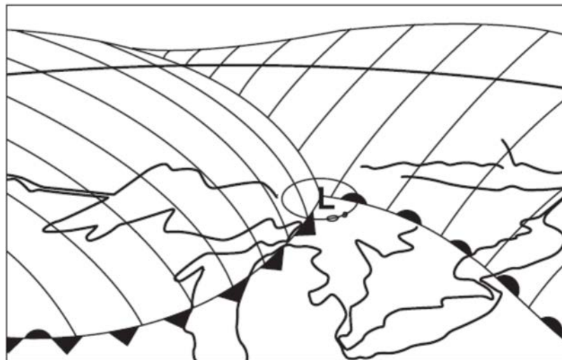
Figure H-1 Occluded Front Formation
