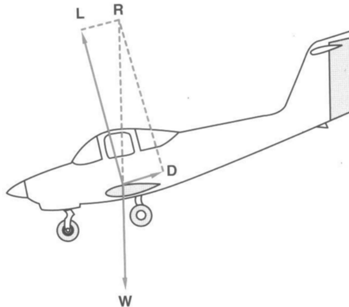
Figure A-5 Forces in a Climb
