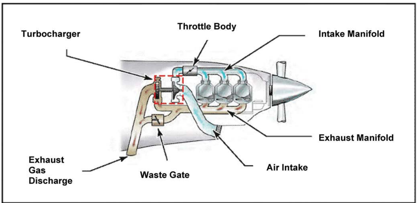
Figure C-1 Turbocharger Components
