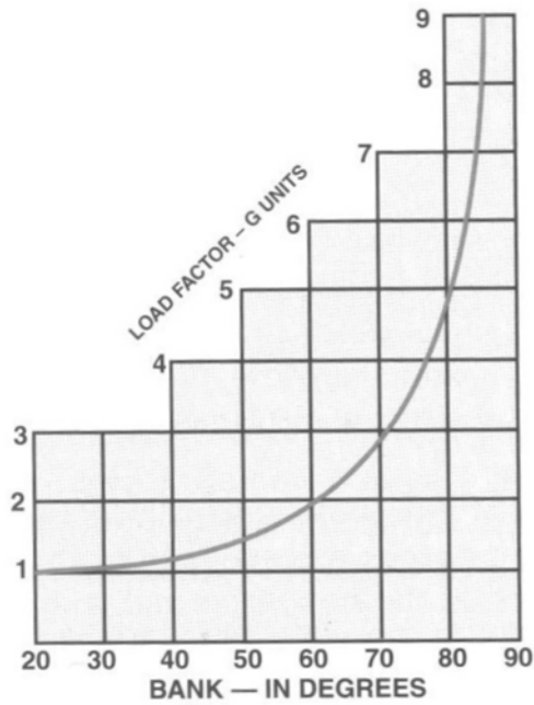
Figure A-7 Forces in a Turn
