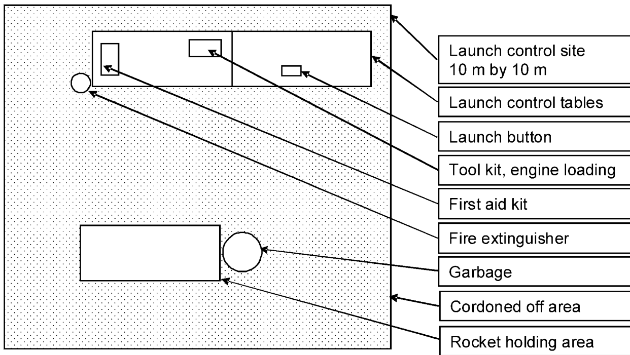
Figure A-1 Layout for a Rocket Launch Site
