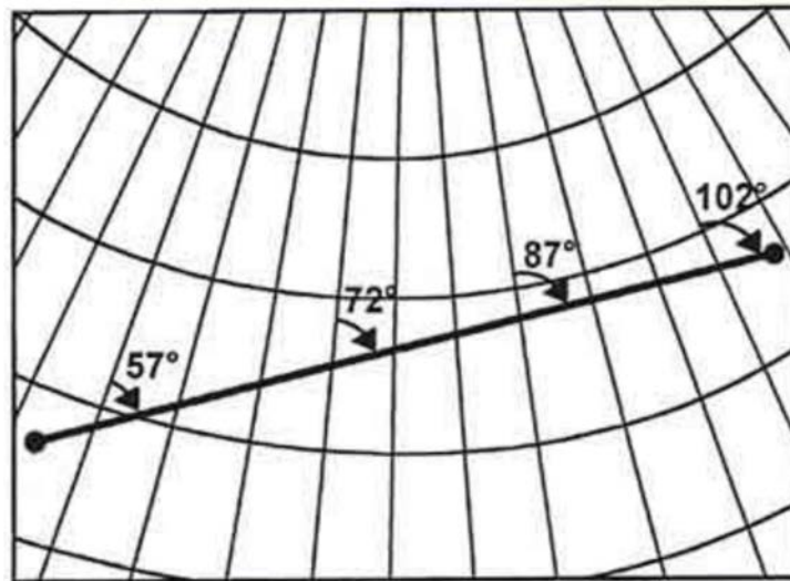
Figure B-1 Great Circle
