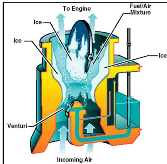
Figure B-1 Float-type Carburetor
