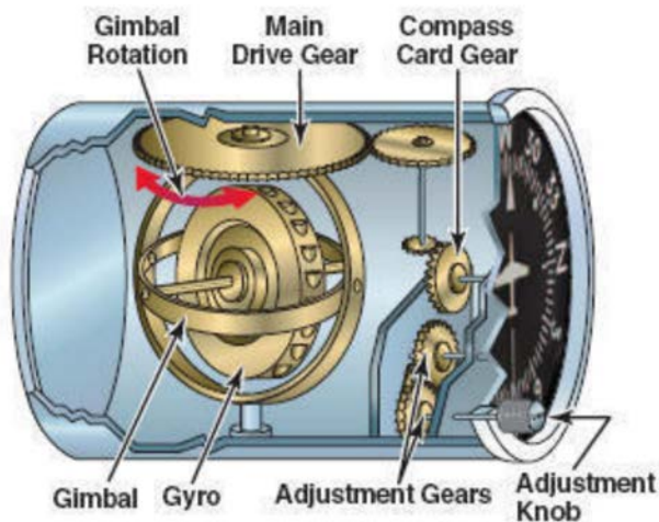
Figure A-5 Gyroscope
