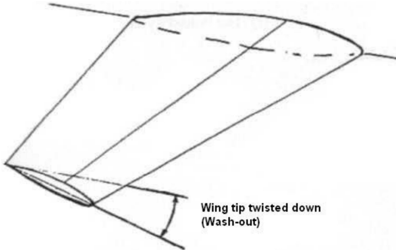
Figure A-6 Wash-Out
