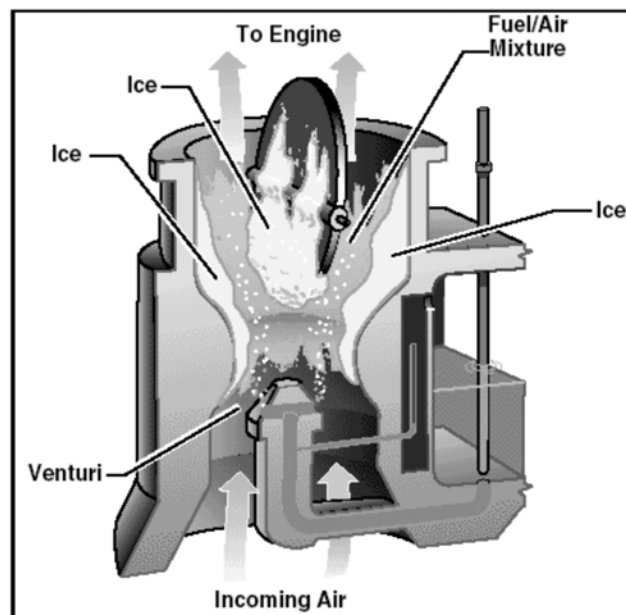
Figure A-5 Float-Type Carburetor
