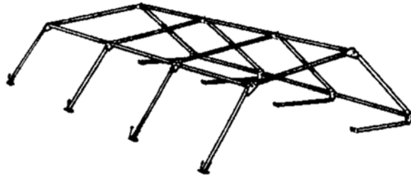
Figure 8 Erect One Side
