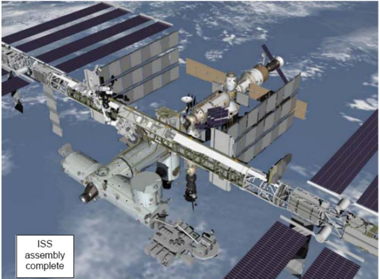
Figure B-2 ISS Truss Structure
