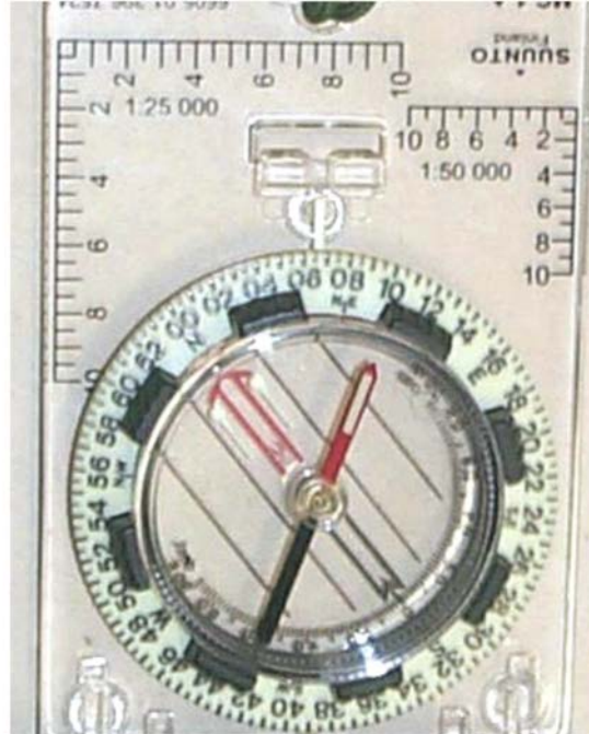
Figure 15 Compass
