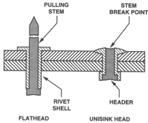
Figure C-3 Pop Rivets
