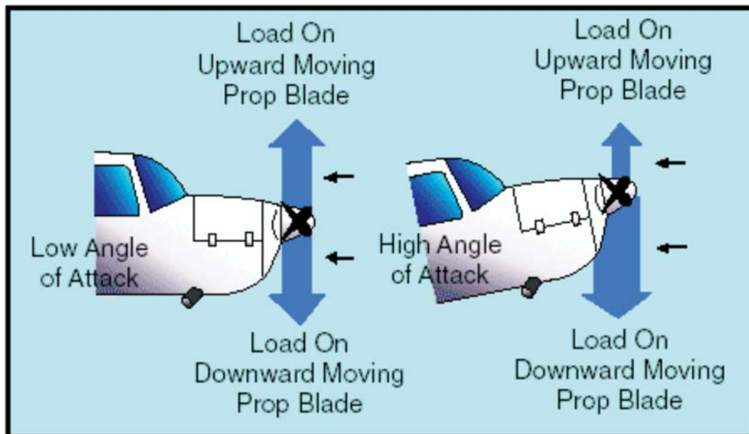
Figure A-1 Torque Reaction
